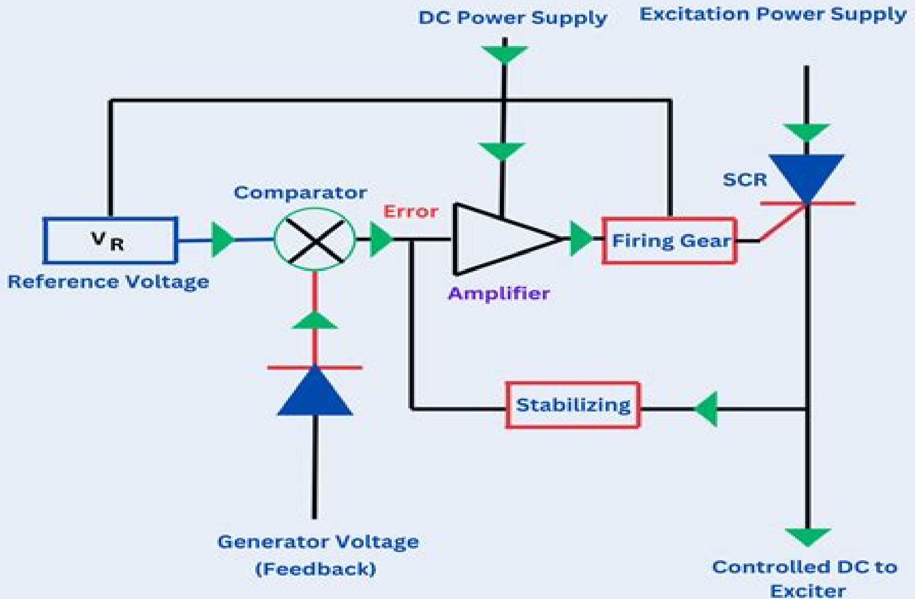
Block Diagram of Automatic Voltage Regulator(AVR))
