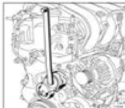
2 Torque tighten the auto tensioner according to (227 Nm) using the:
