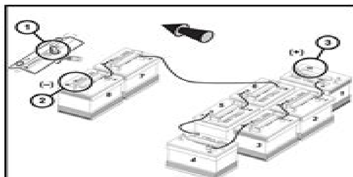
Figure 1-7 Transporter 4 and 6 IQ Plus and Carryall 6 (Style A) IQ Plus Battery Configuration
