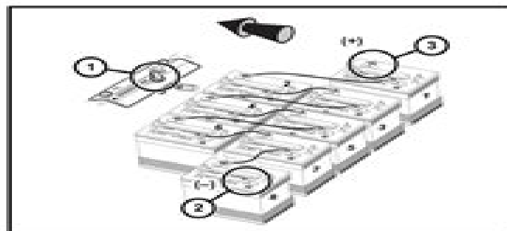
Figure 1-6 Turf 2 and 252/Carryall 2 and 252/ XRT 900 IQ Plus and Carryall 6 IQ Plus (Style B) Battery Configuration
