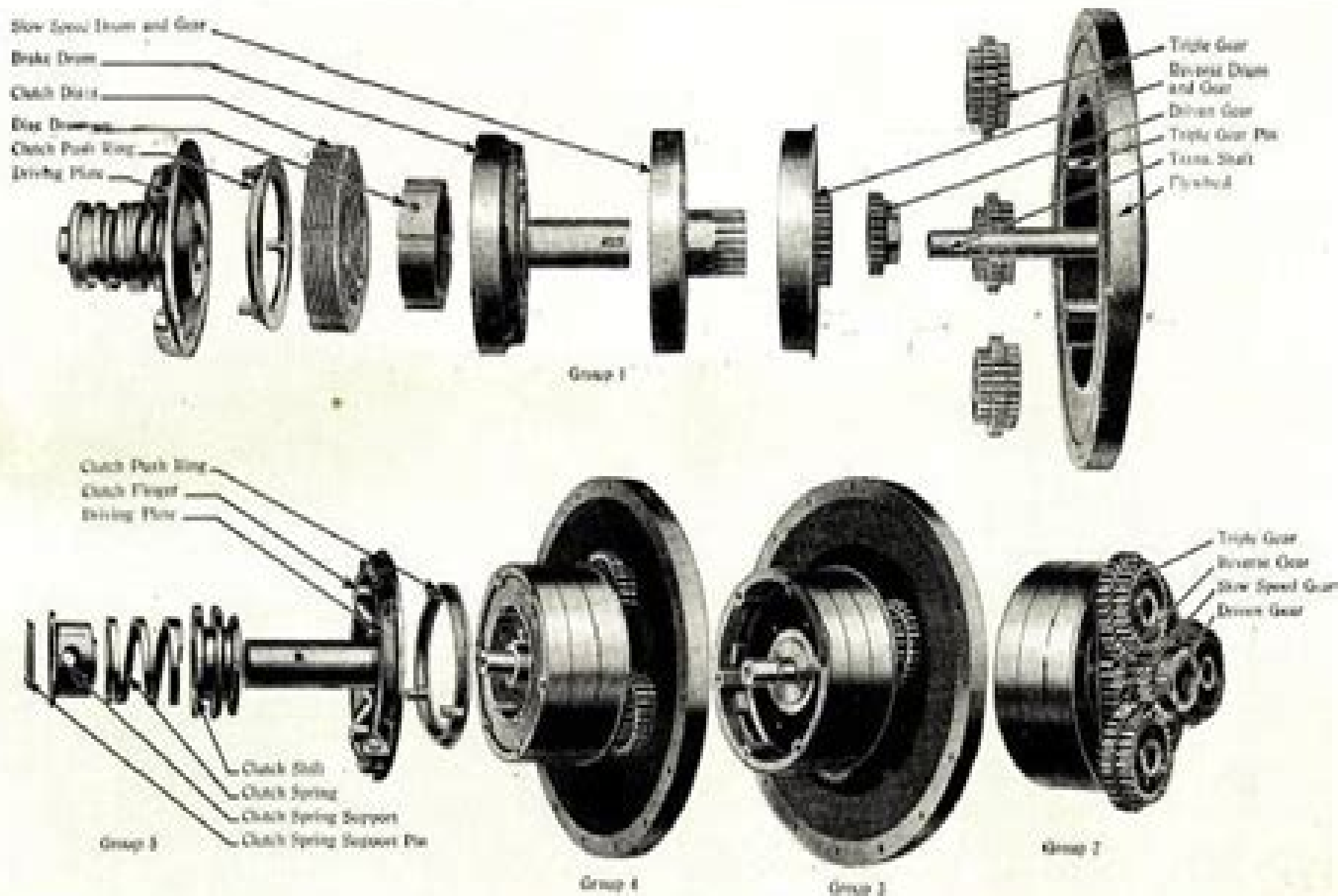
Transmission parts in their relative assembling positions. (Illus. No. 14)
