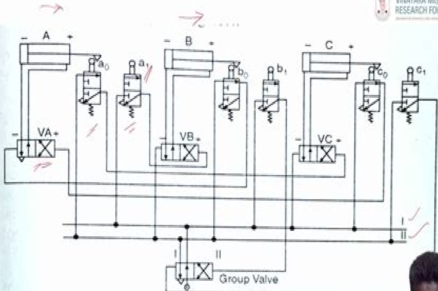
Cascade Circuit for C^+ , A^+ , B^+ , B^+ , A^+ , C^+
