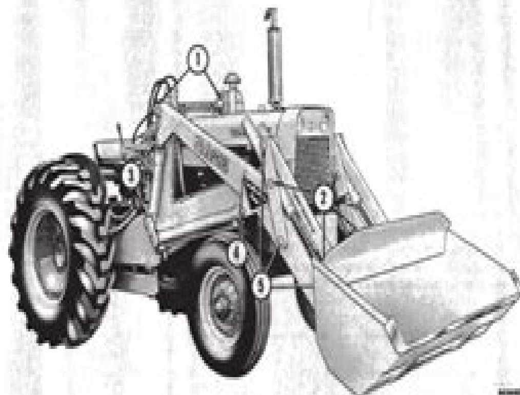
Figure 3 - Loader Pressure Fittings
